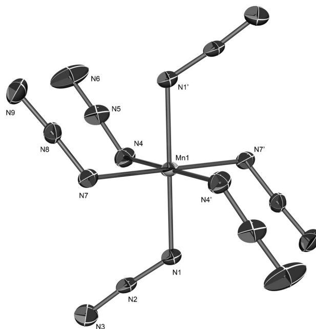
Figure 3. The anion in the crystal structure of [\text{PPh}_4]_2[\text{Mn}(\text{N}_3)_6] . Thermal ellipsoids are shown at the 50% probability level. Selected bond lengths [Å] and angles [°]: Mn1–N1 1.9716(11), Mn1–N4 2.0087(12), Mn1–N7 1.9936(11), N1–N2 1.205(2), N2–N3 1.147(2), N4–N5 1.206(2), N5–N6 1.147(2), N7–N8 1.212(2), N8–N9 1.143(2); N1–Mn1–N1' 180.00(3), N1–Mn1–N4 90.12(5), N1–Mn1–N7 90.53(5).
