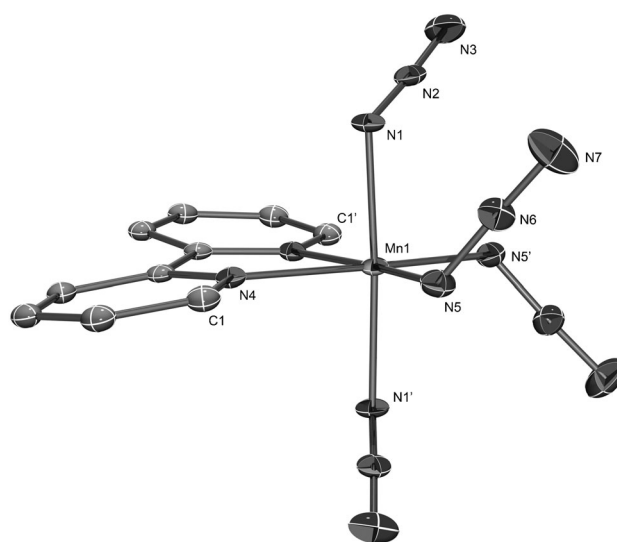
Figure 2. Crystal structure of (\text{bipy})\text{Mn}(\text{N}_3)_4 . Thermal ellipsoids are shown at the 50% probability level. Selected bond lengths [Å] and angles [°]: Mn1–N1 1.9623(13), Mn1–N4 2.0720(13), Mn1–N5 1.9178(14), N1–N2 1.214(2), N2–N3 1.145(2), N5–N6 1.222(2), N6–N7 1.139(2); N1–Mn1–N1' 176.54(8), N1–Mn1–N5 91.71(6), N1–Mn1–N5' 90.59(6).
